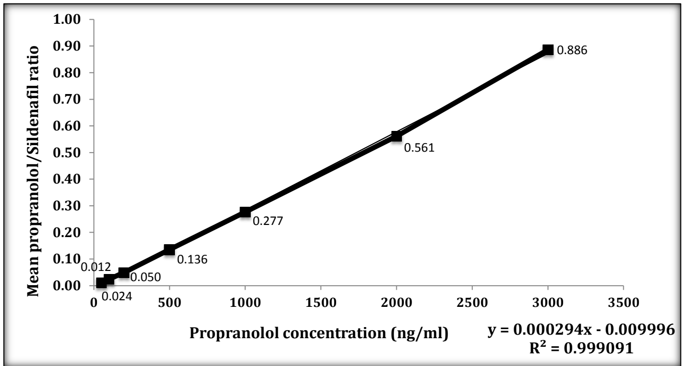
Figure 3.7 Propranolol concentrations versus mean area ratios for each concentration of standard points.
